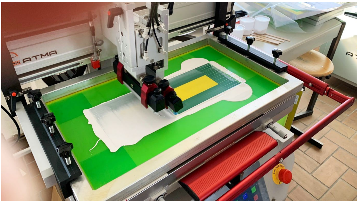
Picture 9: Printing of NoriPUR® highly opaque white screen printing ink
